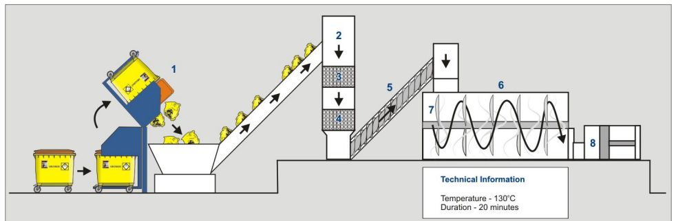
Above: The layout of the Hydroclave Facility
